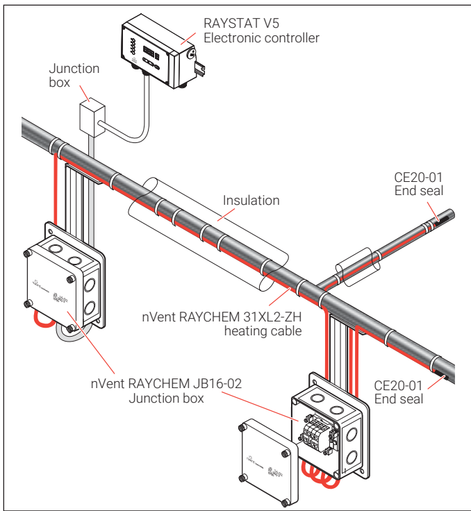
Typical above-ground piping system
