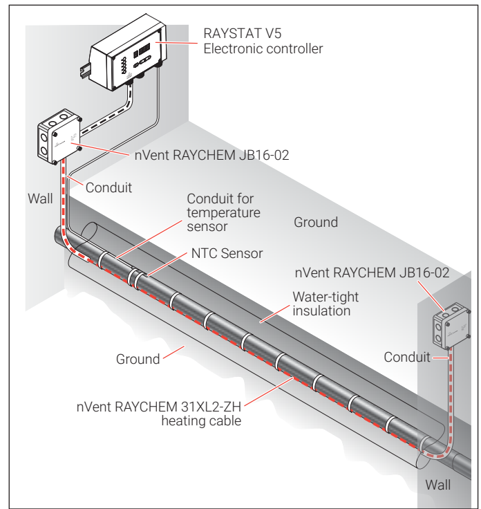
Typical buried piping system
