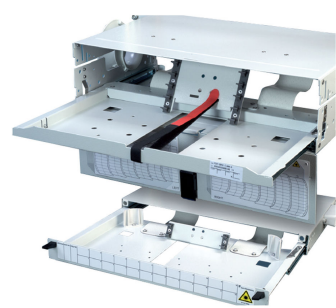
FIST-GPS3 Fiber Panel for holding up to 4 GPST Patch/Splice Trays, unloaded, 2RU, 15 in, gray
